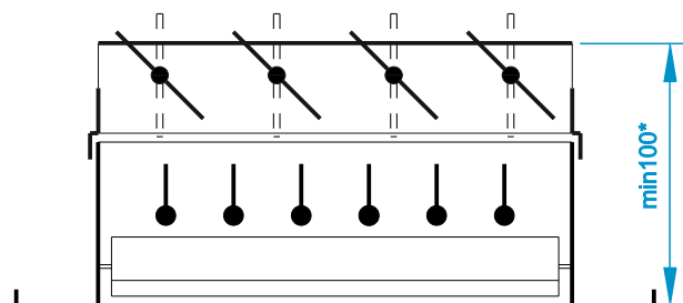
PC7-A-B2, PH7-A-B2
